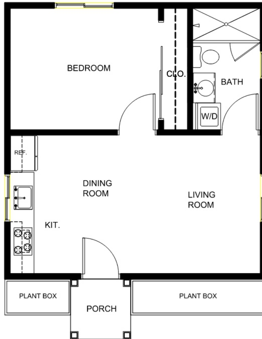
Olfati Design Group - Plan 2 FLOOR PLAN
